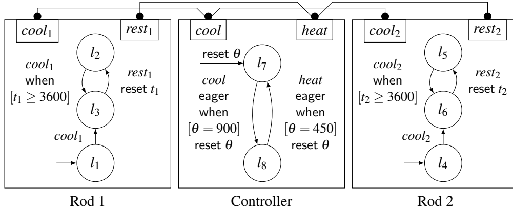
Figure 2: Temperature Control System [4]
