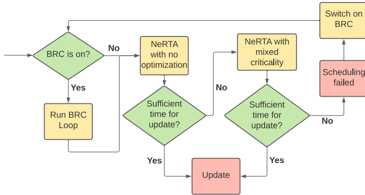
Fig. 12. Choice of optimization to apply. The color choices are the same as in Figure 11 with the addition of red for the final action taken of whether to schedule the update.
